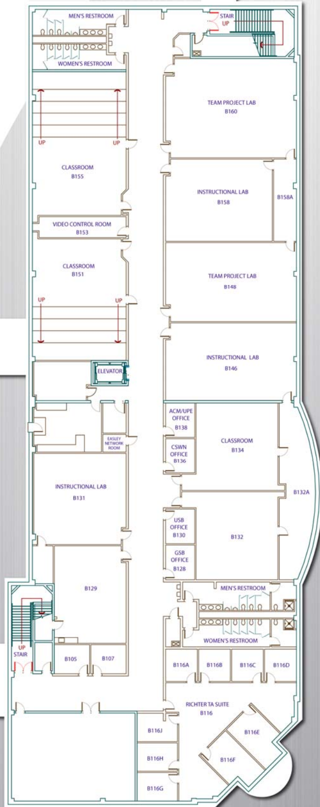
RICHARD AND PATRICIA LAWSON COMPUTER SCIENCE BUILDING LWSN BASEMENT FLOOR PLAN 16 0 16 32 SCALE: 1:16
