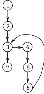
Figure 1: Sums and its control flow graph.
