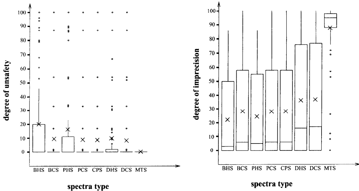
Figure 3: Graphs showing the degrees of unsafety and imprecision of spectra. The vertical axes list degrees of unsafety and imprecision, respectively; the horizontal axes list spectra types. In each boxplot, the dashed line represents the median, and the “X” mark represents the mean, of the degree of imprecision or unsafety that occurred for that spectra. The box indicates the interquartile range – the range in which the middle half of the data falls – and also indicates where that data falls with respect to the median. The whiskers above and/or below boxes indicate the percentages at which data above or below the interquartile range fell; however, data points at a distance of greater than 1.5 times the interquartile range are considered outliers, and represented by small circles.
