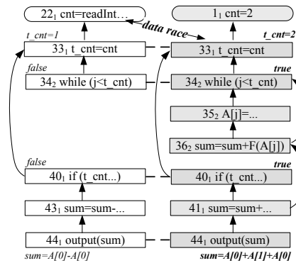
Figure 5: The dual slice of the failure in Fig. 4. A symbol s_i represents the i th instance of statement s in the trace.
