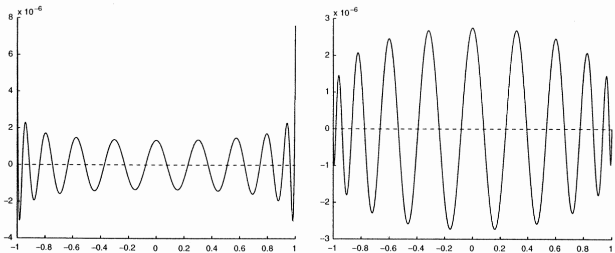
Fig. 3. Legendre vs. Althammer polynomial.
