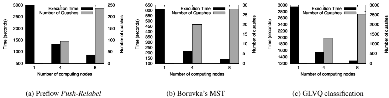
Figure 4. Performance of Preflow Push-Relabel, Boruvka’s MST, and GLVQ classification using CUGS protocol
