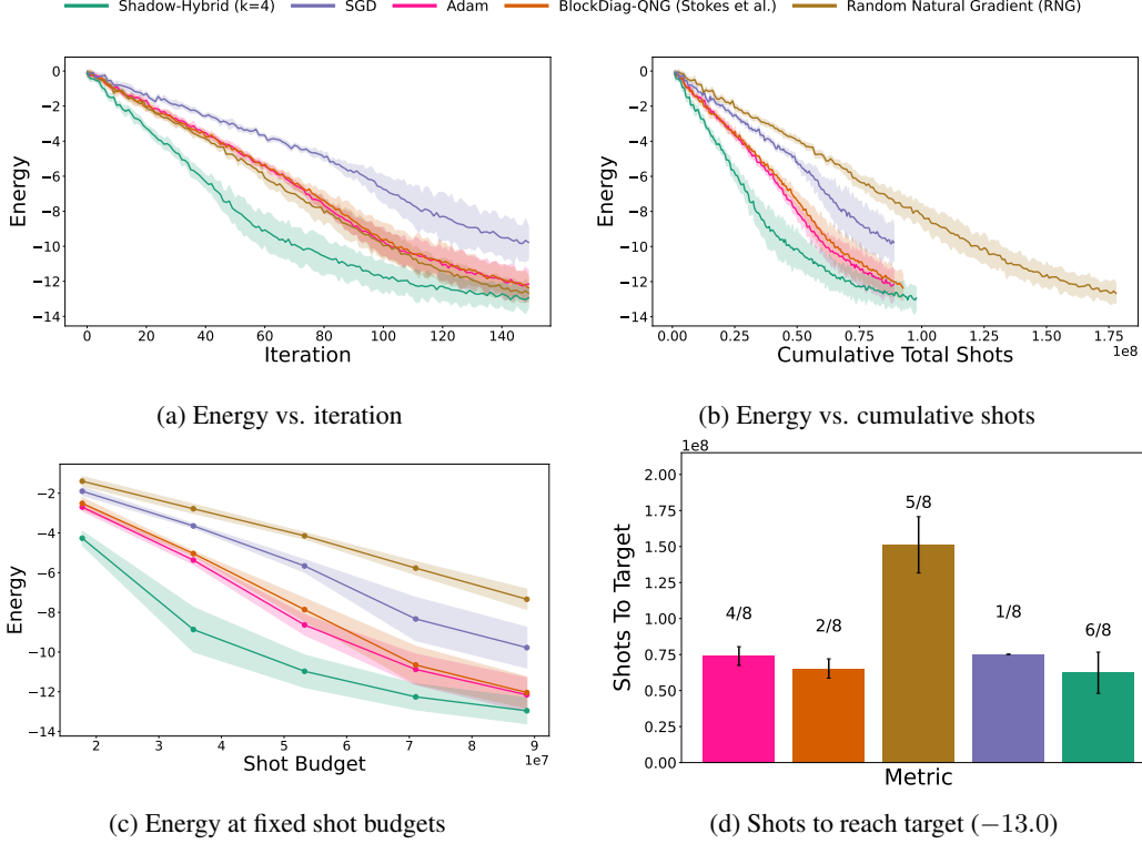
Figure 6: Convergence on the 12-qubit, depth-6 Ising model over 8 matched random seeds. (a) Energy vs. iteration. (b) Energy vs. cumulative shots. (c) Energy at fixed shot budgets. (d) Shots to reach preset benchmark target ( -13.0 ); fractions indicate seeds (out of 8) reaching the target. The target is a fixed threshold, not the true ground-state energy. Shaded bands in (a)–(c) show 95% confidence intervals over seeds. Error bars in (d) show mean \pm SD over successful seeds only.
