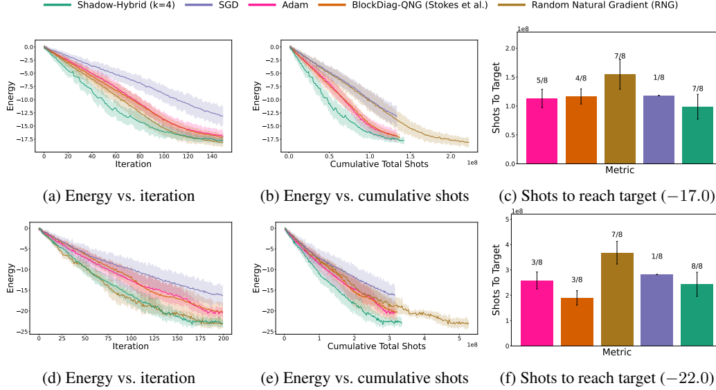
Figure 2: Convergence on 1D Heisenberg chains over 8 matched random seeds. Top row: 12-qubit, depth-6. Bottom row: 16-qubit, depth-8. Columns show energy vs. iteration, energy vs. cumulative shots, and shots to reach a preset benchmark target ( -17.0 for the top row, -22.0 for the bottom row). Shaded bands in the iteration and cumulative shot panels show pointwise 95% confidence intervals over seeds. The shots-to-target panels report mean \pm SD over successful seeds only: fractions above bars indicate the number of seeds reaching the target. Targets are fixed benchmarking thresholds shared across methods and seeds, not true ground-state energies. Energies at fixed shot budgets are reported in Figure 3 (Appendix G.1).
