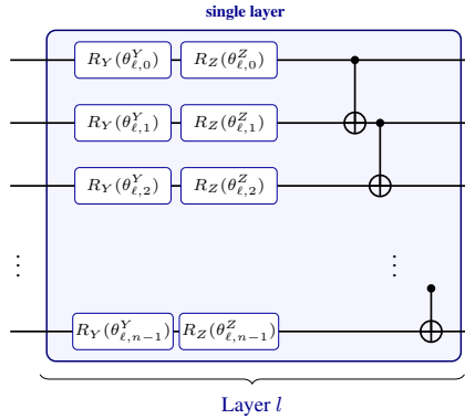
Figure 8: A single layer of the hardware-efficient ansatz used in the experiments. Each layer applies trainable R_Y and R_Z rotations on every qubit, followed by a nearest-neighbor CNOT ladder. The full circuit is obtained by repeating this layer for l = 1, \dots, d .
