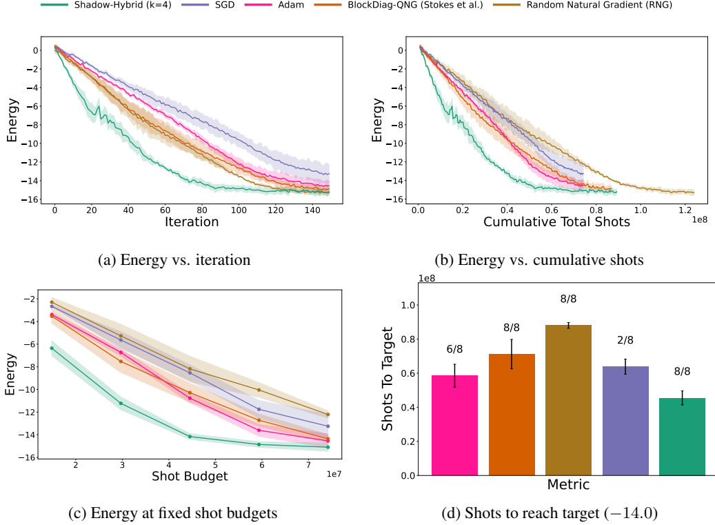
Figure 4: Convergence on the 10-qubit, depth-4 Heisenberg model over 8 matched random seeds. (a) Energy vs. iteration. (b) Energy vs. cumulative shots. (c) Energy at fixed shot budgets. (d) Shots to reach preset benchmark target ( -14.0 ); fractions indicate seeds (out of 8) reaching the target. The target is a fixed threshold, not the true ground-state energy. Shaded bands in (a)–(c) show 95% confidence intervals over seeds. Error bars in (d) show mean \pm SD over successful seeds only.
