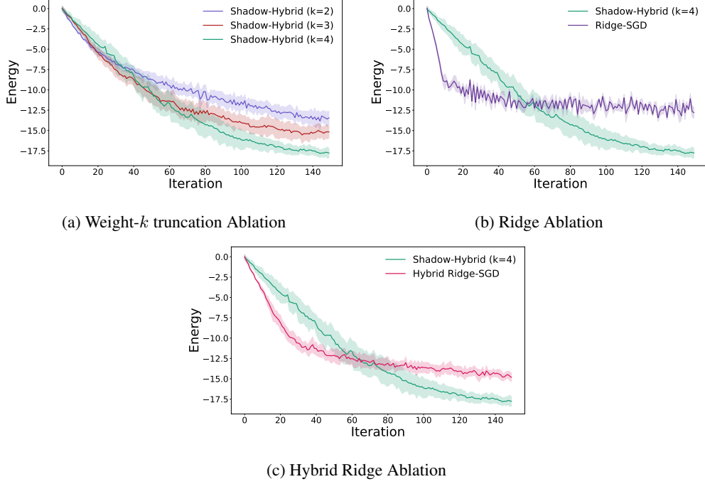
Figure 7: Ablation convergence on 12-qubit, depth-6 1D Heisenberg model over 8 matched random seeds. Shaded bands show 95% confidence intervals over seeds.
