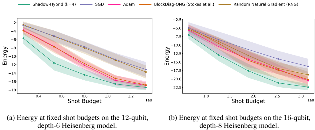
Figure 3: Energy at fixed cumulative shot budgets.
