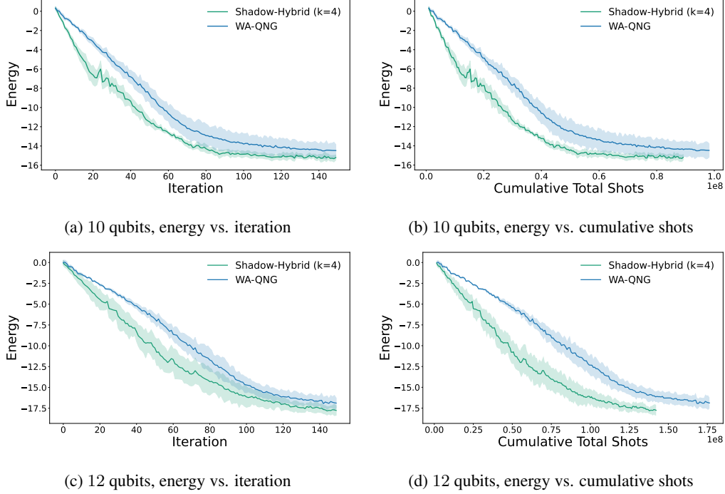
Figure 5: Comparison of Shadow-Hybrid and WA-QNG on the 1D Heisenberg model over 8 matched random seeds. The 10-qubit instance has depth 4, and the 12-qubit instance has depth 6. Shaded bands show 95% confidence intervals over seeds.
