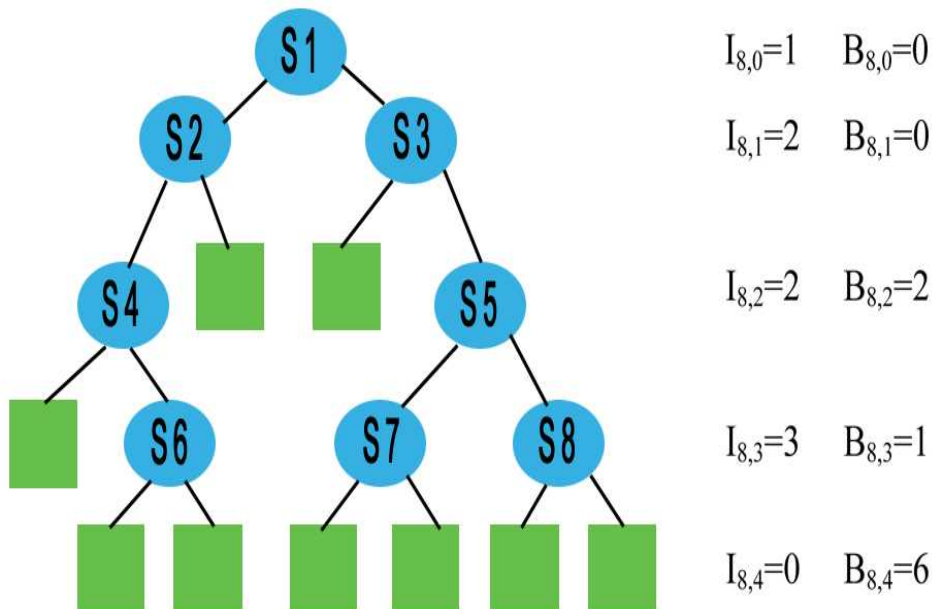
Figure 1: A digital search tree built on eight strings s_1, \dots, s_8 (i.e., s_1 = 0\dots , s_2 = 1\dots , s_3 = 01\dots , s_4 = 11\dots , etc.) with internal (ovals) and external (squares) nodes, and its profiles.
