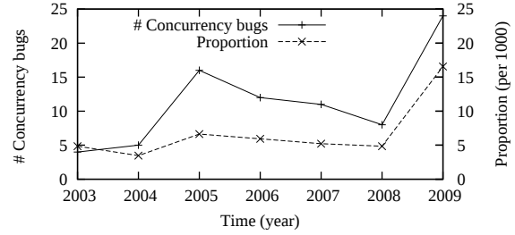
Figure 2. Evolution of bugs (by close date).
