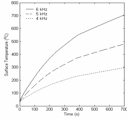
Figure 4: Variation of temperature with heating time (a) at center and outer surface of billet, (b) for various frequency of supply current
