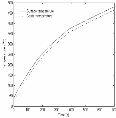
Figure 4: Variation of temperature with heating time (a) at center and outer surface of billet, (b) for various frequency of supply current
