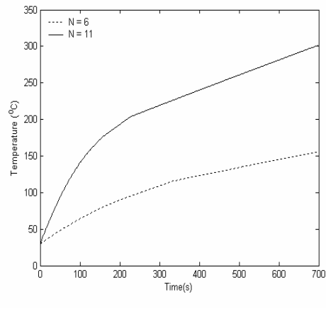
Figure 5: Variation of temperature with time (a) for various amplitude of supply current, (b) for two number of turns of the coil
