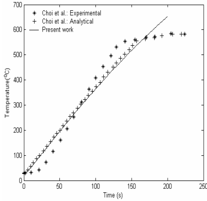
Figure 3: (a) Comparison of predicted temperature rise with time at outer surface of the billet, (b) corresponding temperature distribution for f = 5 \text{ kHz} and I = 200 \text{ A} , N = 6 at t = 200 \text{ s}
