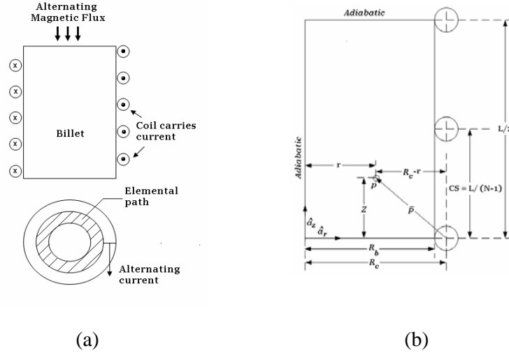
Figure 1: (a) Schematic diagram of induction heating system, (b) Computational domain
