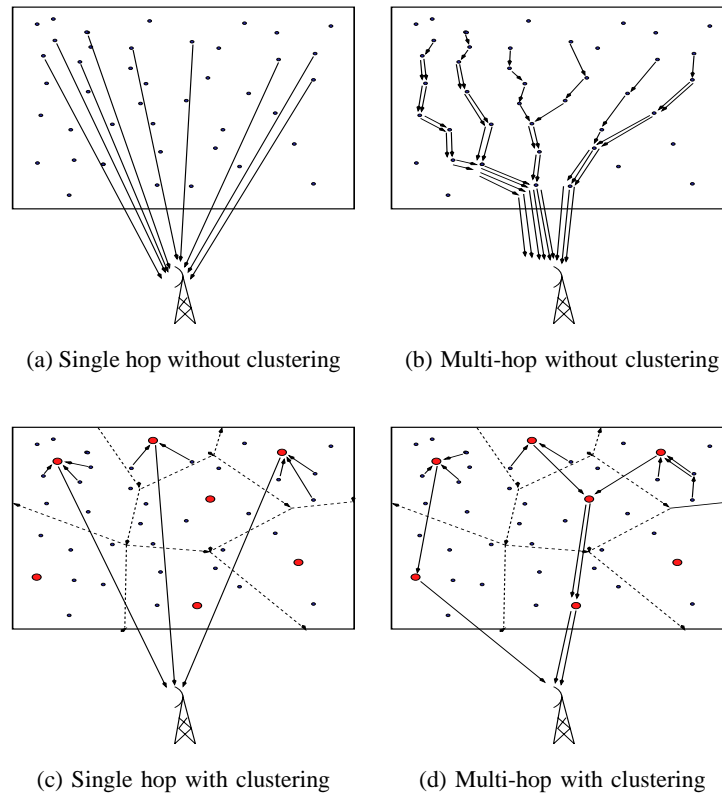
Fig. 1. Sensor information forwarding with and without clustering and aggregation
