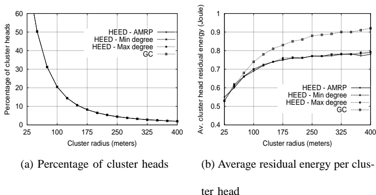
Fig. 4. Characteristics of selected cluster heads
