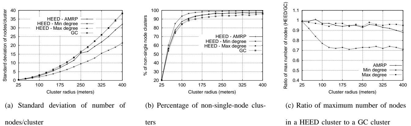
Fig. 5. Characteristics of clusters
