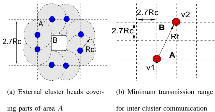
Fig. 3. Conditions on transmission range for network connectivity
