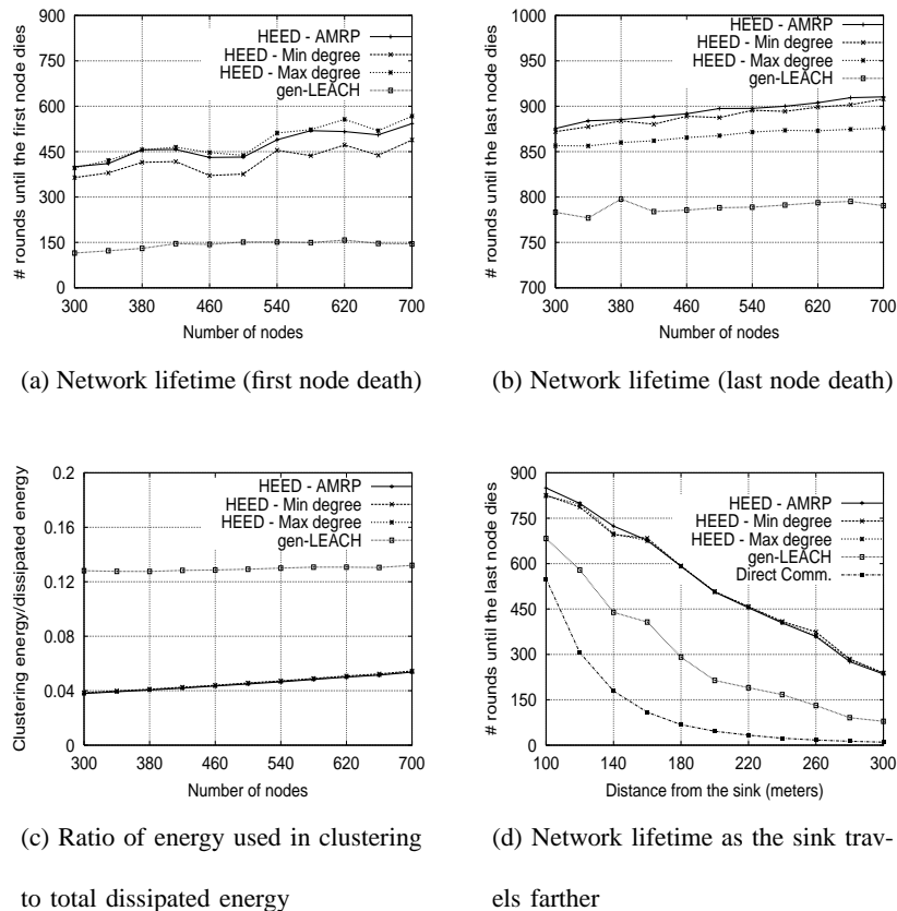
Fig. 8. Performance of HEED on network applications
