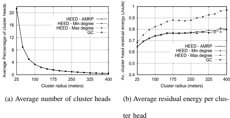
Fig. 7. Clustering quality with non-uniform node distribution
