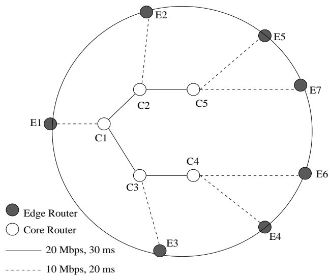
Figure 3: Topology used in simulations. All edge routers are connected to multiple hosts.
