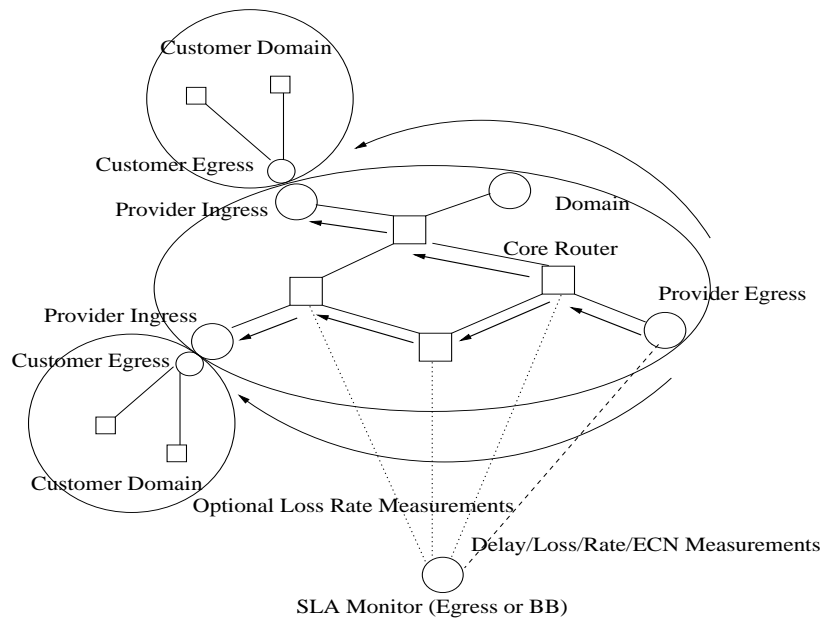
Figure 1: An architecture for detecting SLA violations and bandwidth theft attacks. Assistance from core routers is optional.
