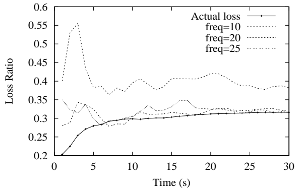
(a) Inferred loss at various probing frequencies
