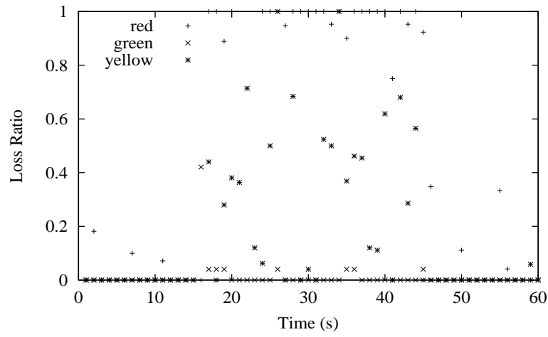
Figure 7: Loss of probe packets in the presence of high excess traffic. Green probes see high loss when a severe attack starts. Yellow and Red probes experience high drops as expected
