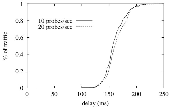
(a) Delay for different probe frequencies
