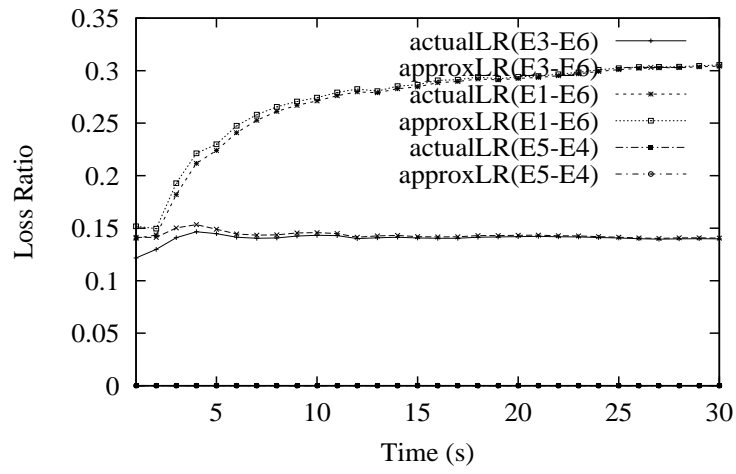
Figure 6: Loss approximation with the core-assisted scheme.
