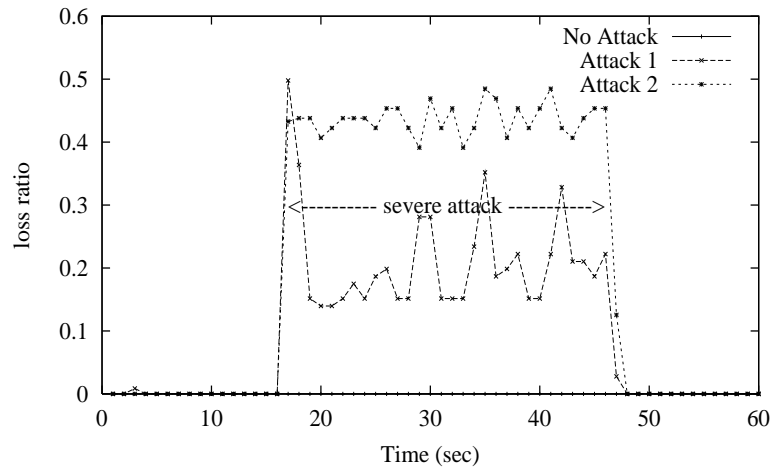
Figure 11: Overall loss follows the same pattern as delay
