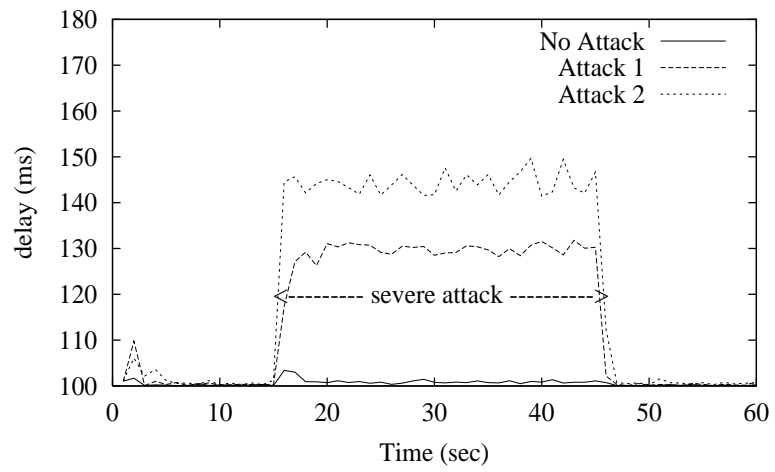
Figure 10: Observed delay at the time of an attack. “Attack 1” results in packet loss in excess of 15-25%. “Attack 2” increases packet loss to more than 35%
