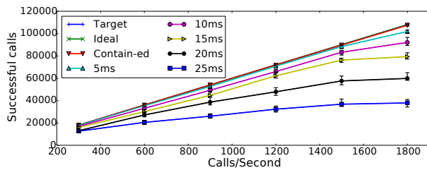
Figure 4: Successful REGISTER calls
