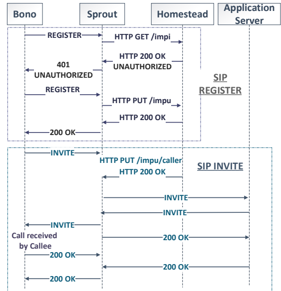
Figure 2: Clearwater IMS Call Flow
