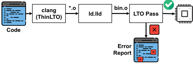
Fig. 5: Compilation and Analysis pipeline for CRT-C.
