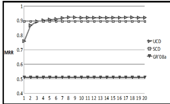
Fig. 5: Comparison between supervised and unsupervised models, tested on English-Hebrew NE pairs. We show the learning curves for Hebrew under two different settings: unsupervised (denoted UCD) and supervised (denoted SCD). The model presented in [Goldwasser & Roth 08a] (denoted GR08a) is also included here. Note that our unsupervised model outperforms the supervised model, trained with 250 labeled examples. See the text for more comparisons and details.
