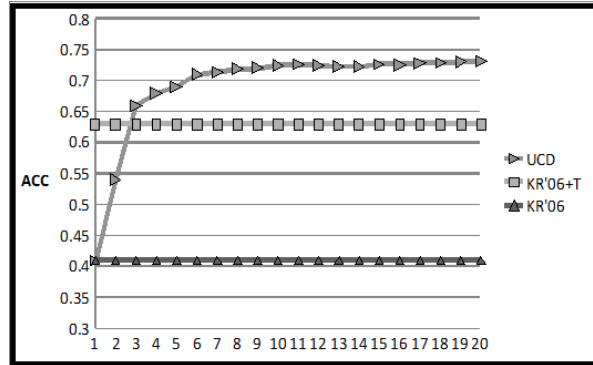
Fig. 2: Comparison between our model (denoted UCD ) and weakly supervised learning methods [Klementiev & Roth 06b]. Note that one of the models proposed in [Klementiev & Roth 06b] takes advantage of the temporal information. Our best model, the unsupervised learning with all constraints, outperforms both models in [Klementiev & Roth 06b], even though we do not use any temporal information.
