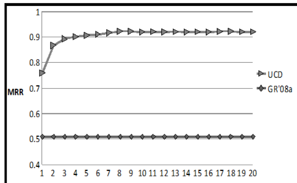
Fig. 3: Comparison between supervised and unsupervised models, tested on English-Hebrew NE pairs. We show the learning curve for the unsupervised version of our model (denoted UCD), tested on the English-Hebrew dataset. We compare it to the supervised model presented in [Goldwasser & Roth 08a] (denoted GR08a). Results show a significant improvement when using our model
