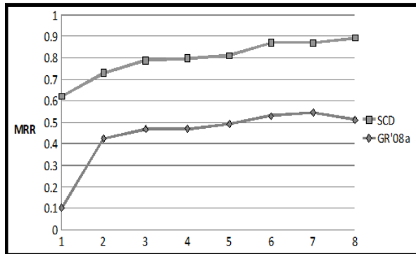
Fig. 4: Comparing our method (denoted as SCD in the graph) to [Goldwasser & Roth 08a] over the English-Hebrew data, using different training sets. Results show that using as little as 10 labeled examples our method can outperform a system trained using 250 labeled examples.
