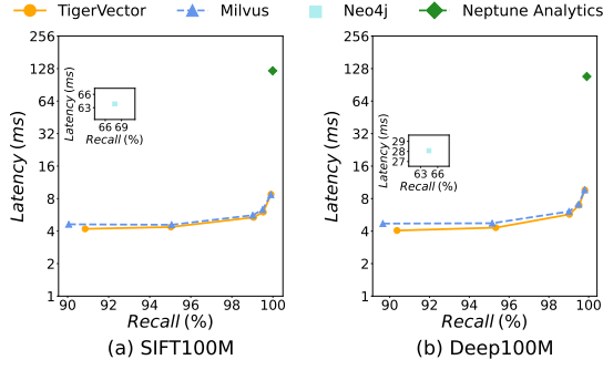
Figure 8: Latency Evaluation on SIFT100M and Deep100M
