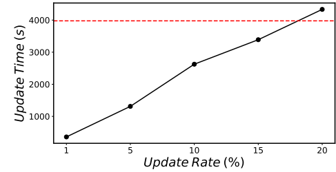
Figure 11: Index Update Evaluation on SIFT100M
