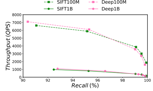
Figure 10: Data Size Scalability
