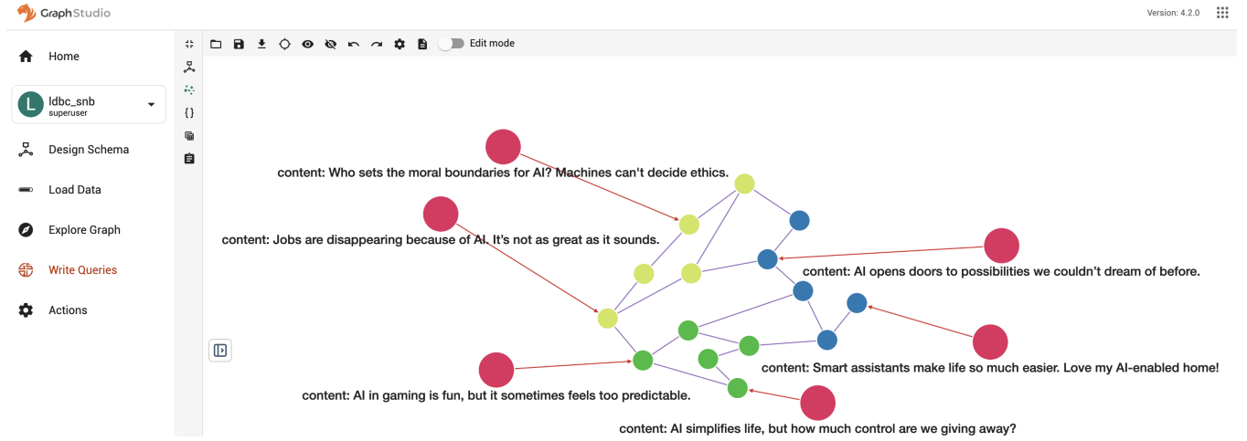
Figure 6: Demonstration of Combining Community Detection and Vector Search. The Person vertices are partitioned into three communities, colored green, blue, and yellow. The top-k Posts from each community are colored red.
