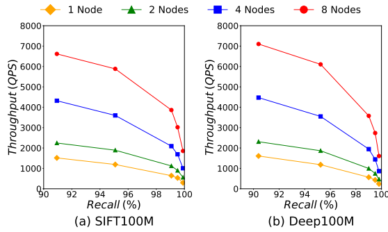
Figure 9: Node Scalability
