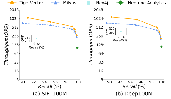
Figure 7: Throughput Evaluation on SIFT100M and Deep100M
