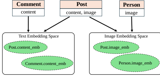
Figure 2: Example of Embedding Space
