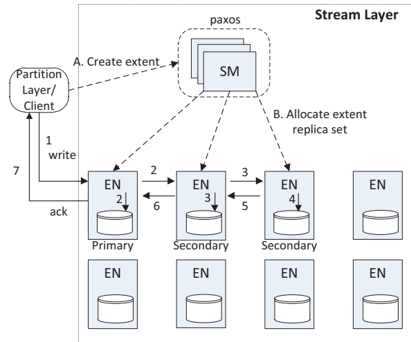
Figure 3: Stream Layer Architecture
