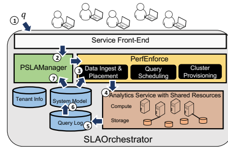
Figure 2: SLAOrchestrator Architecture.
