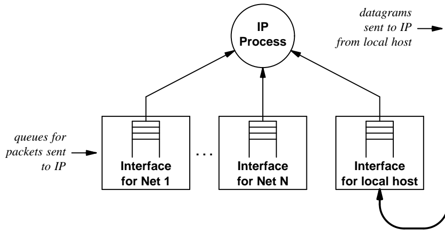
Figure 5.1 IP must select a datagram for processing from the queues associated with network interfaces. The pseudo-network interface provides a queue used for datagrams generated locally.
