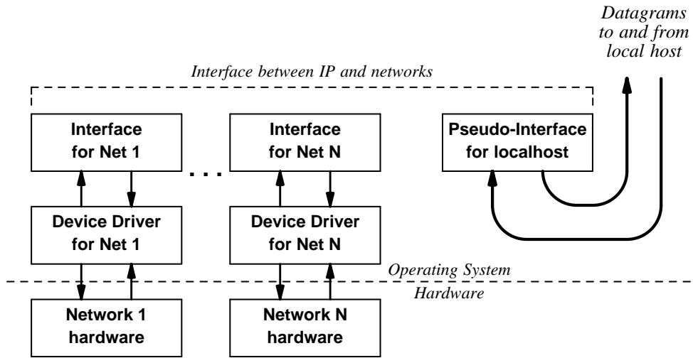
Figure 3.2 The pseudo-network interface used for communication with the local host.
