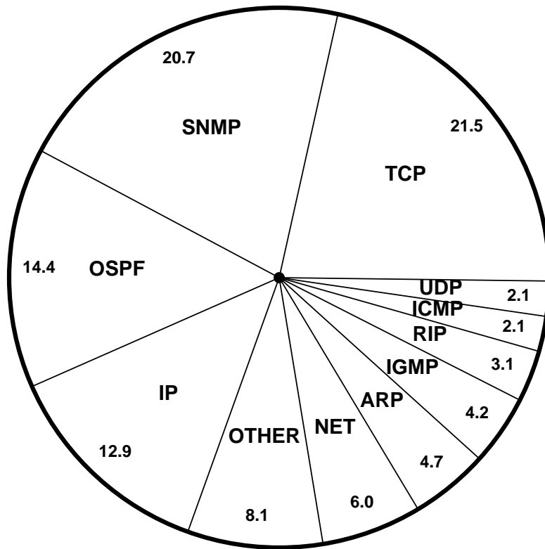
Figure 25.2 Number of functions and procedures used to implement each protocol as a percentage of the total. The chart displays protocols in decreasing number of procedures.
