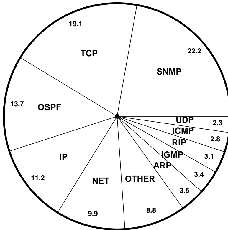
Figure 25.1 Lines of code used to implement each major protocol as a percentage of the total. Category OTHER includes miscellaneous utility functions, such as the one used to compute checksums, as well as initialization code.
