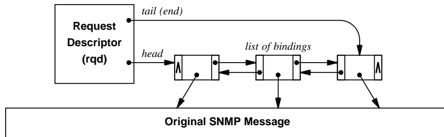
Figure 22.1 The data structure created by snparse . Each node on the binding list corresponds to a MIB variable. The node points to the ASN.1 object identifier found in the original message.
