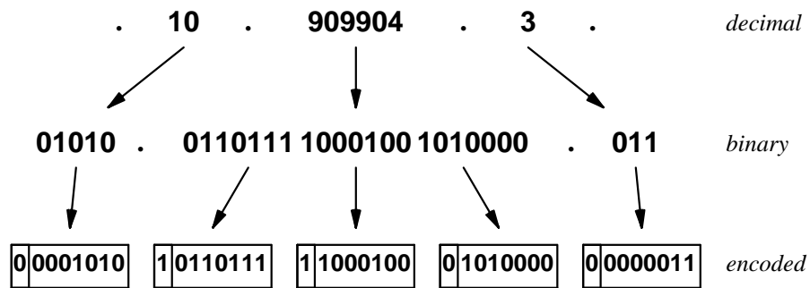
Figure 21.5 Part of an ASN.1 object identifier, shown in decimal, binary, and encoded form. The ASN.1 encoding uses multiple octets to encode integers greater than 127. A zero in the high-order bit of an octet marks the end of a subidentifier.
