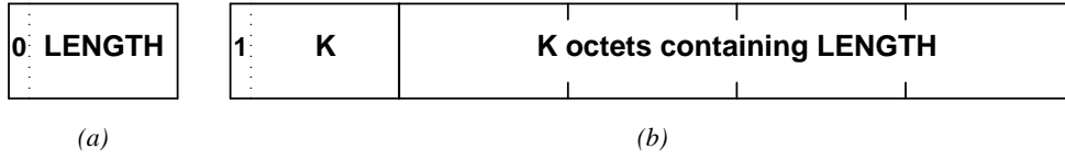
Figure 21.4 The ASN.1 encoding of object lengths. The short form in (a) is used to represent lengths less than 128, while the long-form in (b) is used to represent longer lengths. The high-order bit of the first byte distinguishes the two forms.
