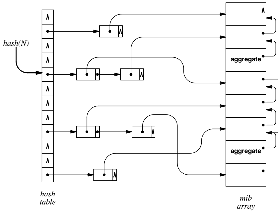
Figure 21.3 The mib array and hash table snhtab that speeds MIB variable lookup. Arrows on the right hand side show lexical links used for get-next-requests ; the lexical order skips nonleaf items.
