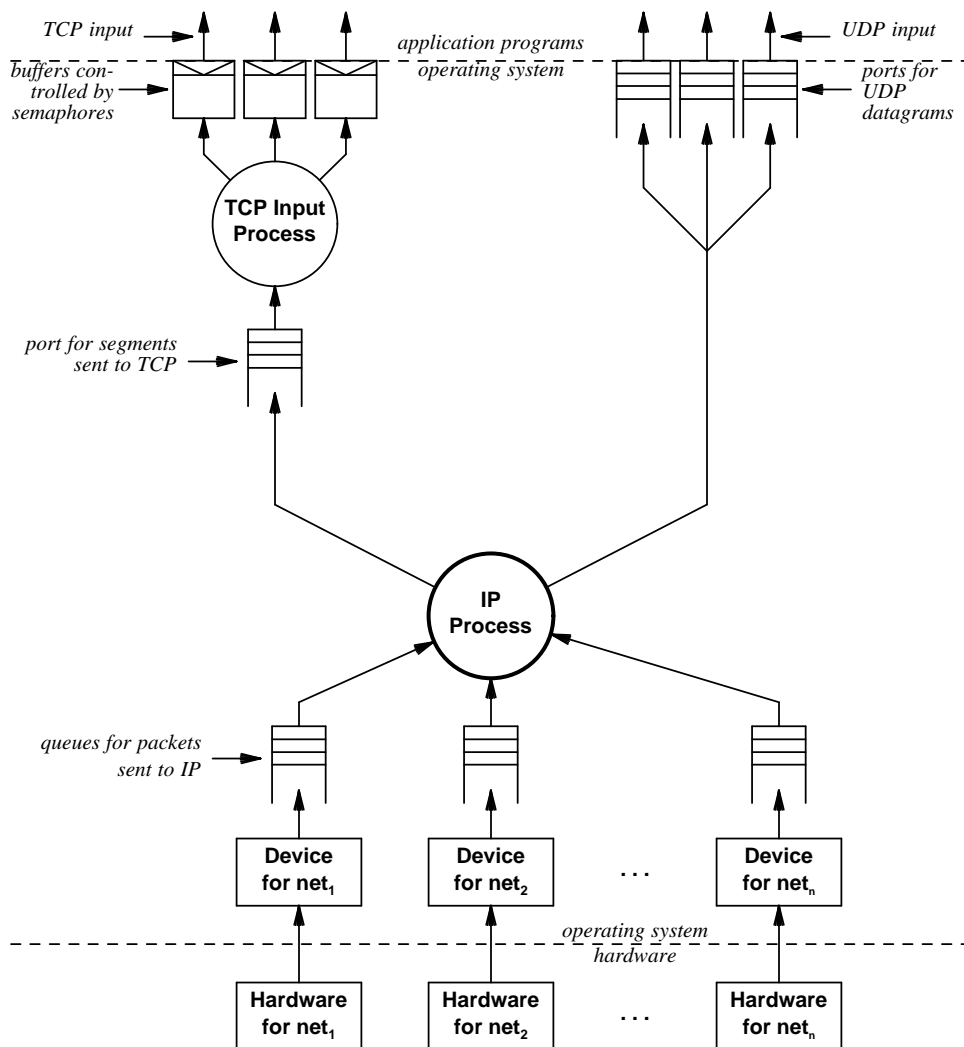
Figure 2.7 Input process structure showing the path of data between the network hardware and an application program. Input to the device queues occurs asynchronously with processing. IP is a central part of the design the software for input and output share a single IP process.
