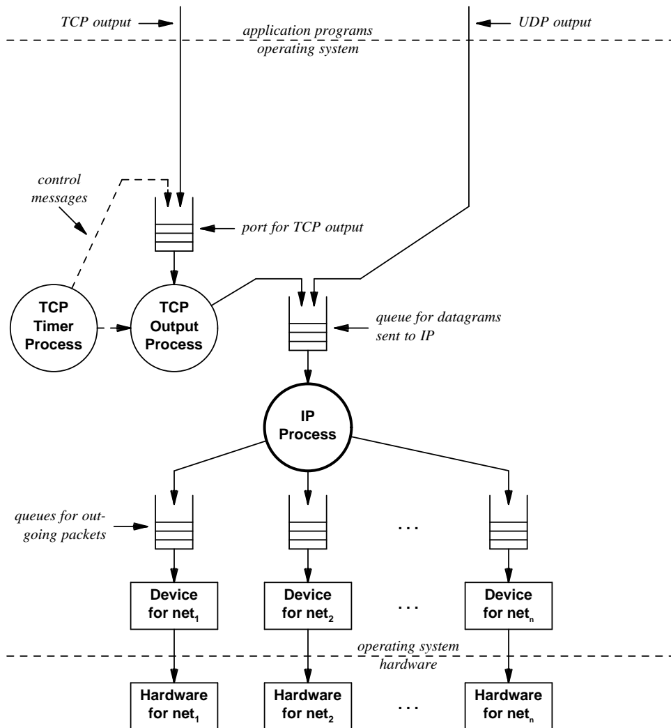
Figure 2.6 Output process structure showing the path of data between an application program and the network hardware. Output from the device queues is started at interrupt time. IP is a central part of the design the software for input and output both share a single IP process.
