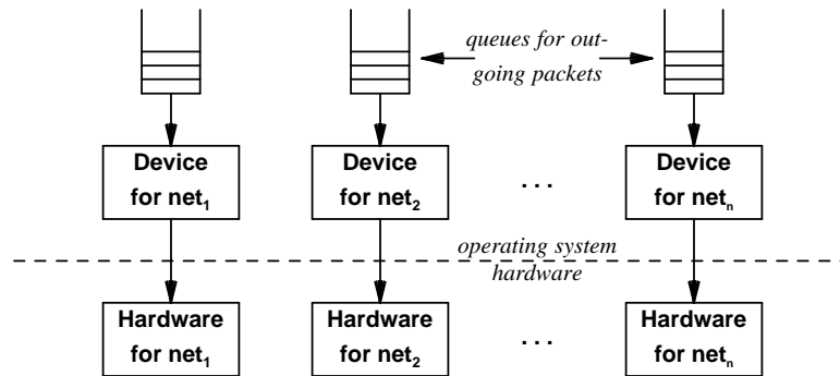
Figure 2.4 Network output and the queues that buffer output packets. Using queues isolates processing from network transmission.
