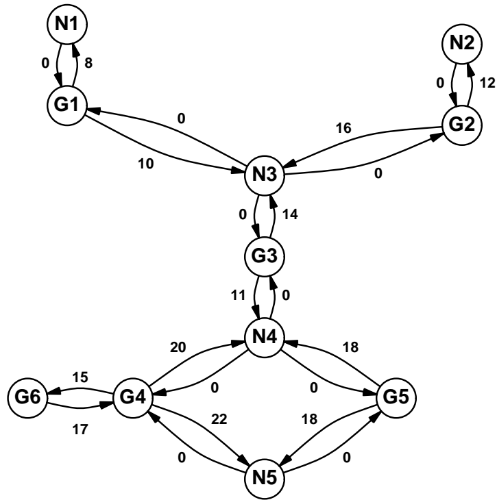
Figure 19.4 The OSPF graph for the internet in Figure 19.3. The number on an edge in the graph corresponds to the weight assigned to the network connection that it represents.
