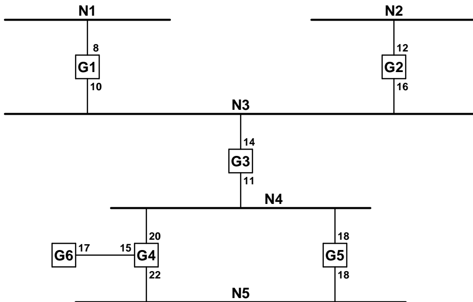
Figure 19.3 An example internet of networks and gateways with costs assigned to each interface.
