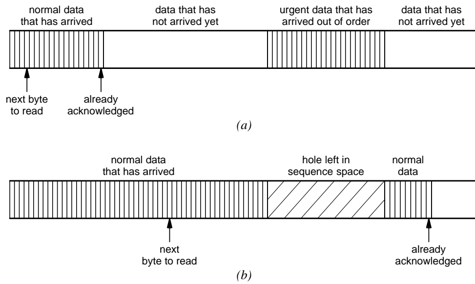
Figure 16.1 (a) The TCP sequence space when urgent data arrives before all normal data, and (b) the same sequence space after urgent data has been processed and additional normal data has arrived. The space occupied by urgent data forms a hole in the space.
