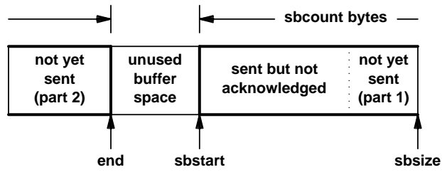
Figure 13.4 Available data wrapped around a circular TCP output buffer. Variable sbcoun tells the number of available bytes and end gives the location of the last byte of data. End can be computed as (sbstart + sbcoun) \bmod sbsize .
