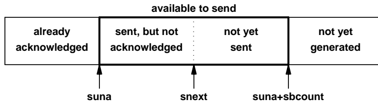
Figure 13.3 The conceptual sequence space and fields in the TCB that maintain pointers into it. Sequence numbers increase from left to right.
