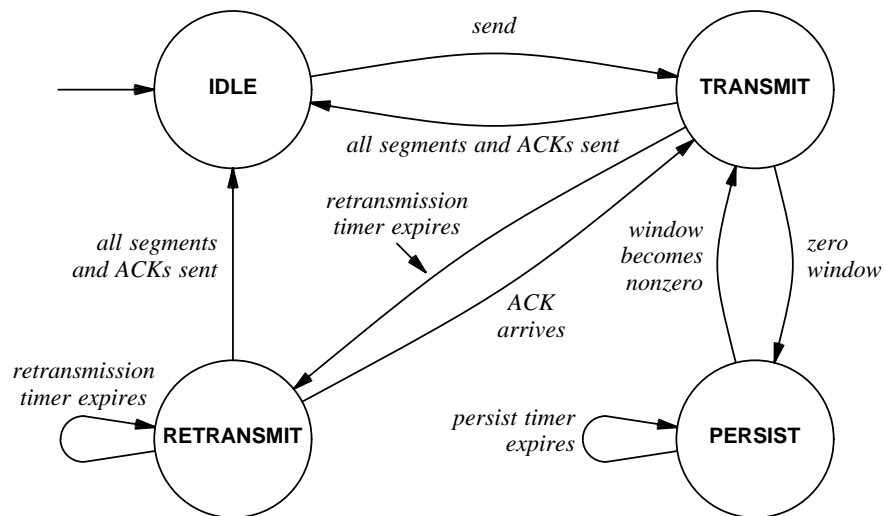
Figure 13.1 Conceptual transitions among the four TCP output states. Unlike the finite state machine used for input, the output state machine is not specified by the TCP protocol standard it was defined for our implementation.
