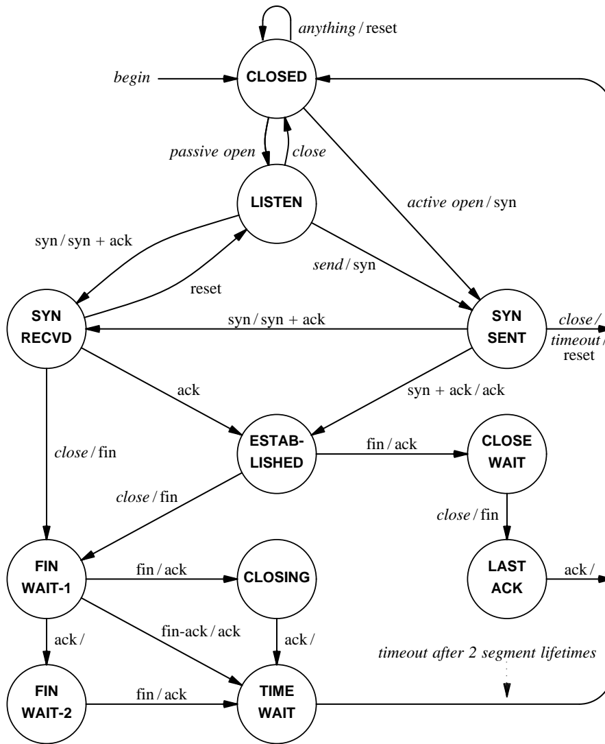
Figure 11.2 The TCP Finite State Machine that controls processing.
