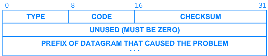
Figure 9.7 ICMP destination unreachable message format.
