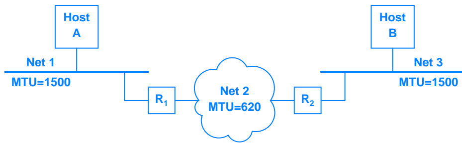
Figure 7.10 An illustration of IPv4 fragmentation. Each router may need to fragment datagrams before sending across network 2.
