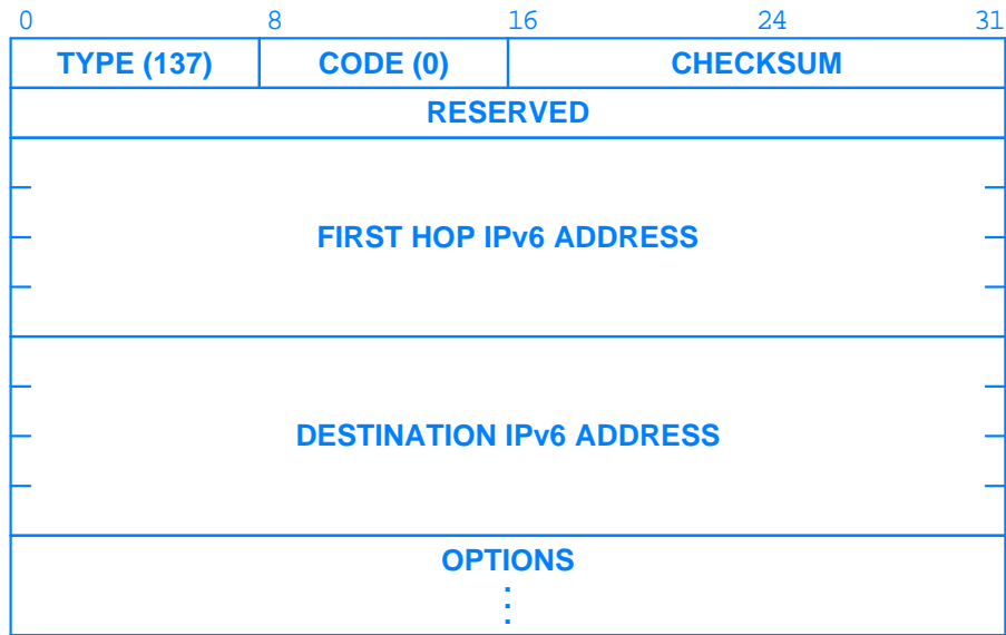
Figure 22.10 The format of an ICMPv6 Redirect message.
