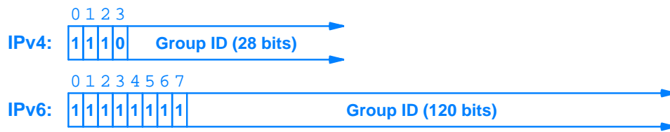
Figure 15.1 The format of IPv4 and IPv6 multicast addresses. A prefix identifies the address as multicast.
