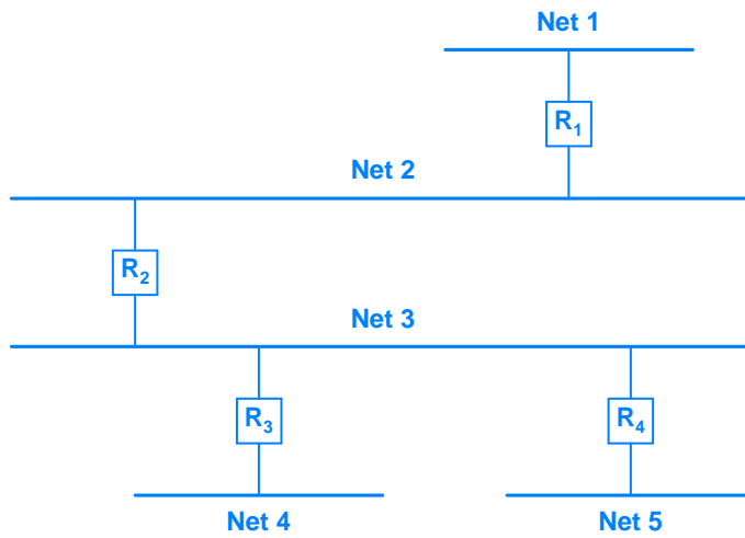
Figure 14.1 An example of a small intranet consisting of five networks and four routers. Only one possible route exists between any two hosts in the example.
