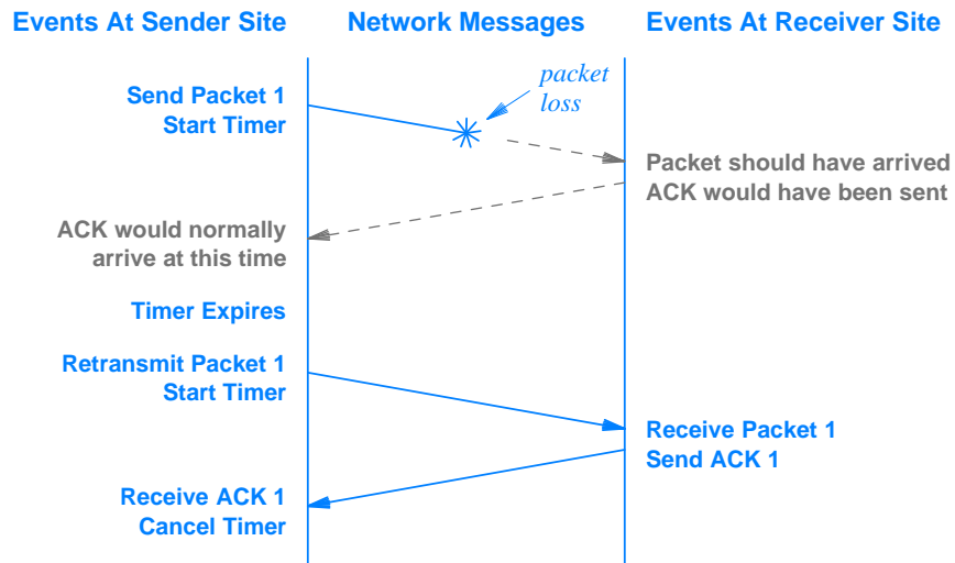
Figure 11.2 Illustration of timeout and retransmission when a packet is lost.
