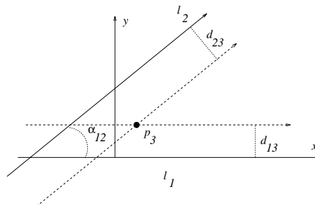
Figure 11: Placing a point relative to two known lines
