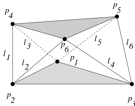
Figure 21: A Stewart platform with triangular platforms
