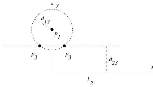
Figure 10: Placing a point relative to a known point and line
