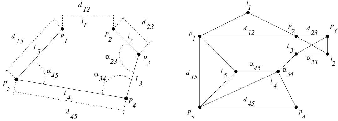
Figure 7: A well-constrained sketch and its constraint graph
