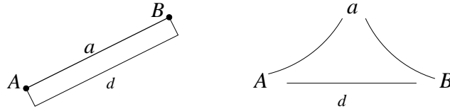
Figure 6: A set of geometric elements with constraints, and the corresponding constraint graph; d denotes a distance constraint.
