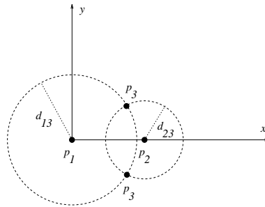
Figure 9: Placing a point relative to two known points
