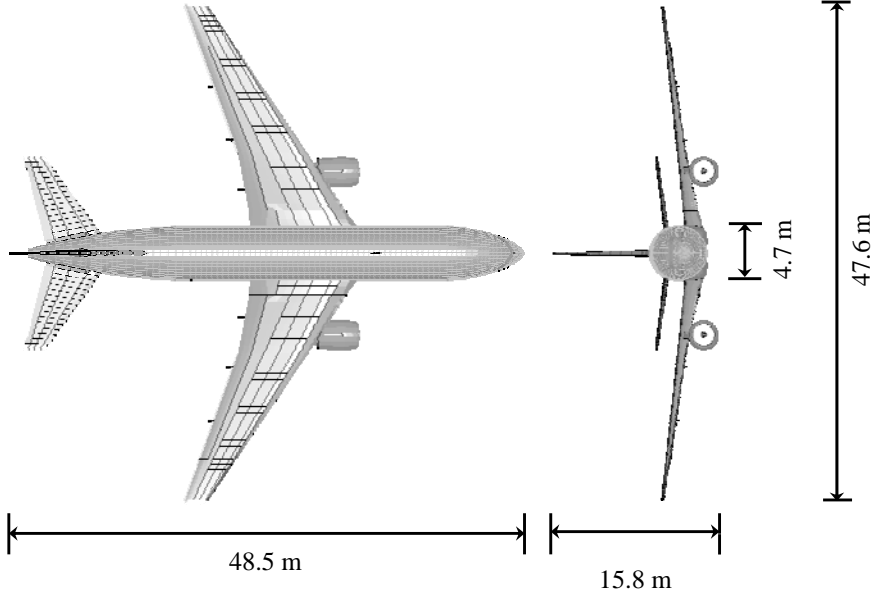
Figure 1. Overall dimensions of Boeing 767-200ER.
