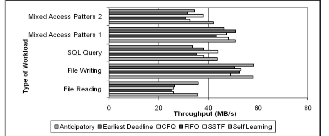
Fig. 11. Average throughput of the self-learning I/O scheme.
