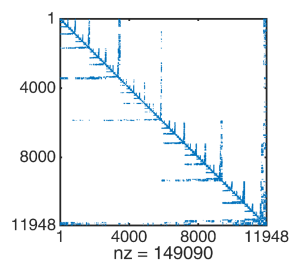
(b) original reordered matrix
