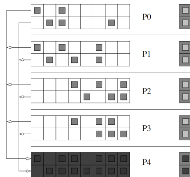
Controlling density of augmented blocks by combining blocks (first row at each processor is combined into first row of the augmented block). Note the reduced fill. Matvec is still tolerant to one process failure.
