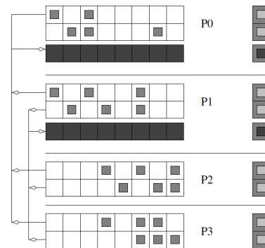
Augmentation block is now distributed across processors. This addresses problem of load imbalance. Note higher communication cost of this scheme. This can be amortized through coarse-grained processor partitions.
