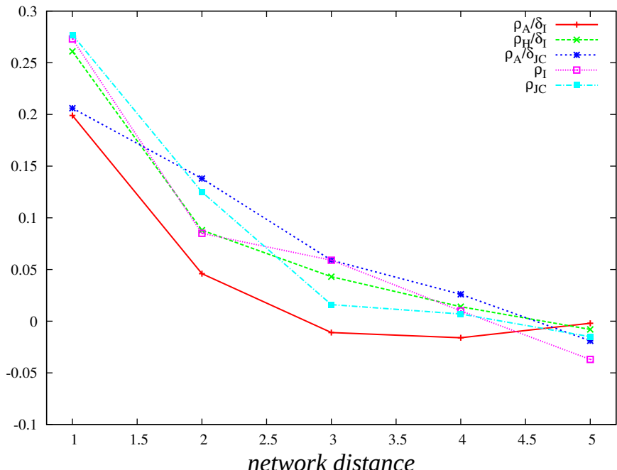
average semantic similarity
