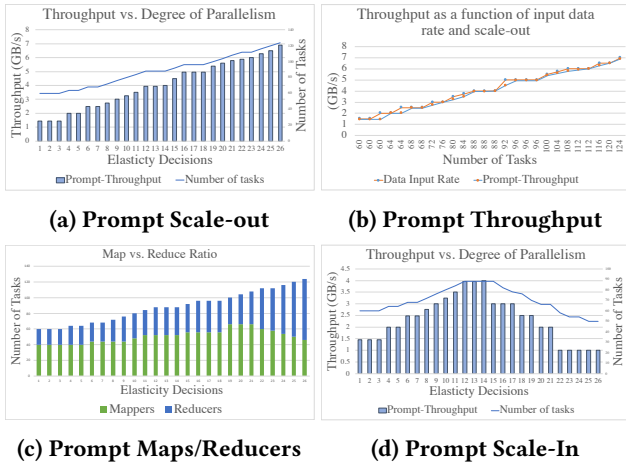
Figure 12: Prompt Elasticity
