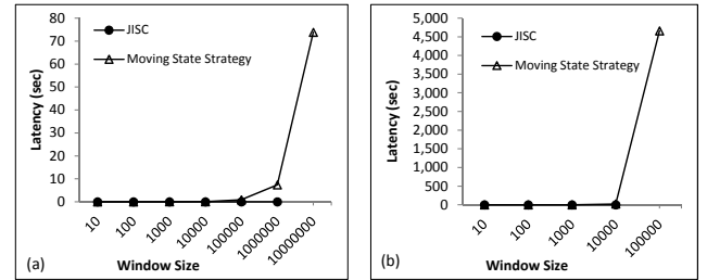
Figure 10: Output latency due to a plan transition. (a) QEP of hash joins. (b) QEP of nested-loop joins.
