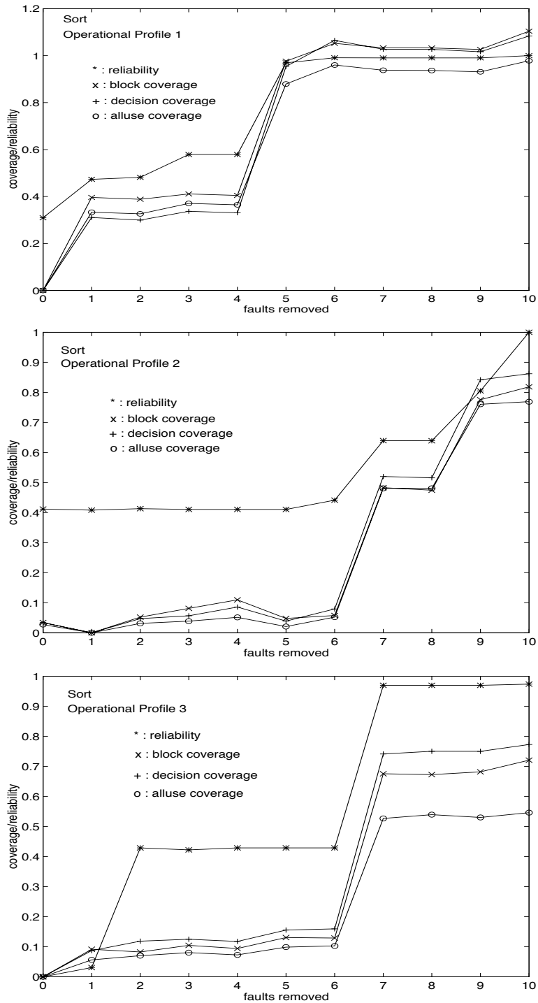
Figure 3: Coverage and reliability versus faults detected for three operational profiles of Sort.
