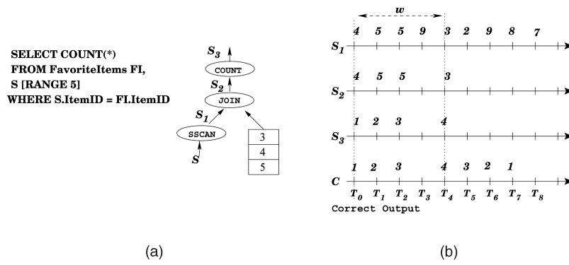
Fig. 1. Input-triggered evaluation. (a) Query Q1 with the query pipeline. (b) Execution timeline.
