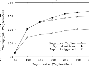
Fig. 10. Throughput for query Q2.
