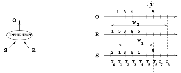
Fig. 3. Window intersection in ITA.
